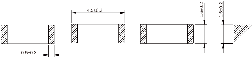
Dimensions: [mm]
